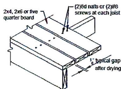
Figure 22 TYPICAL DECKING
