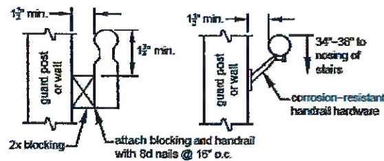
Figure 34 HANDRAIL GRASPABILITY
