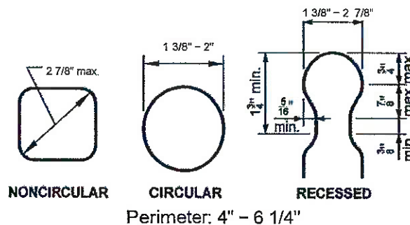
Figure 34 HANDRAIL GRASPABILITY
