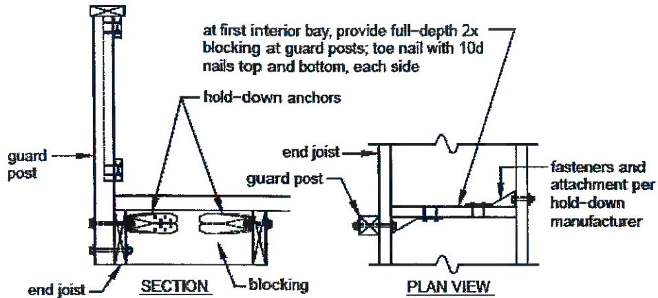
Figure 26 GUARD POST TO RIM JOIST
