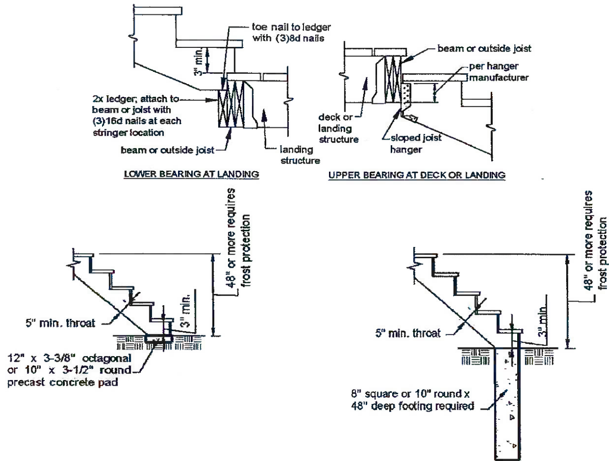
Figure 28 STRINGER BEARING
