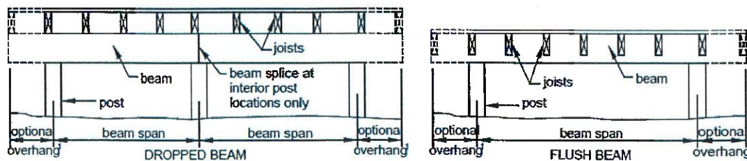
Figure 3 BEAM TYPES
