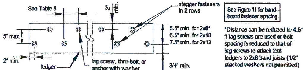
Figure 15 LEDGER BOARD FASTENER SPACING AND CLEARANCES
