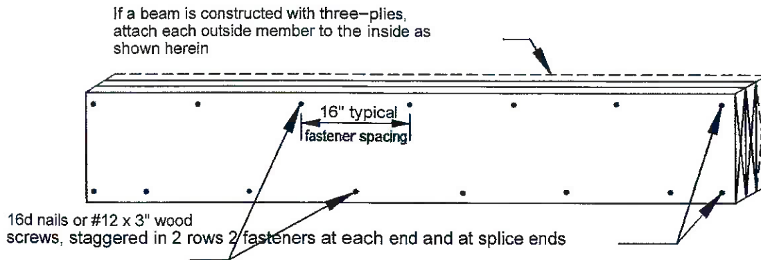
Figure 4 BEAM ASSEMBLY
