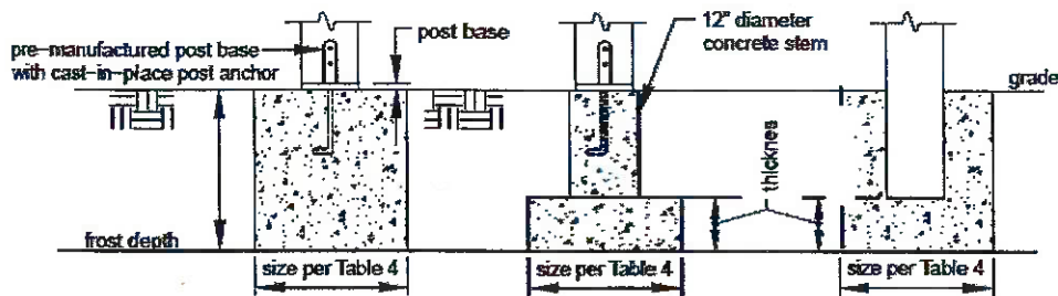
Figure 1 FOOTINGS
