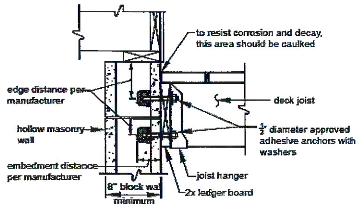
Figure 13 ATTACHMENT OF LEDGER BOARD TO HOLLOW FOUNDATION
