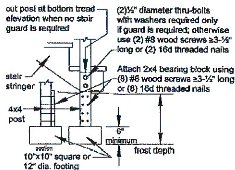
Figure 29 STRINGER BEARING
