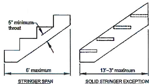
Figure 30 STRINGER SPAN LENGTH
