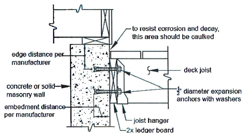
Figure 12 ATTACHMENT OF LEDGER BOARD TO SOLID FOUNDATION
