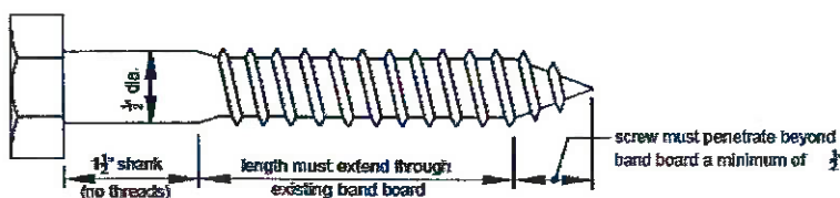
Figure 16 LAG SCREW
