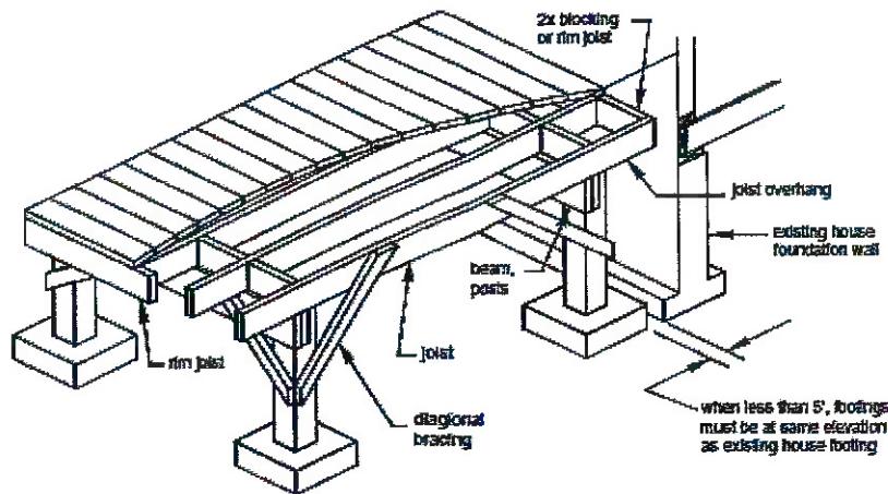
Figure 17 FREE-STANDING DECK
