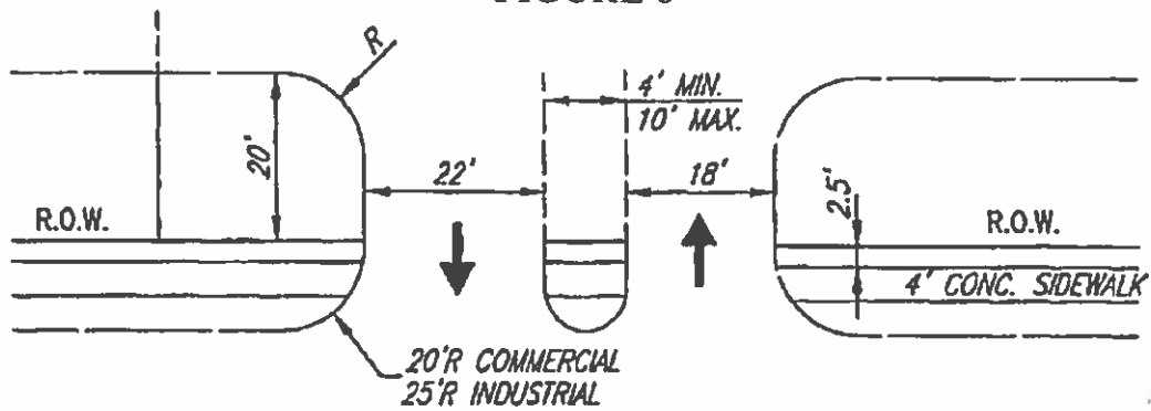
DRIVEWAYS WIDTH, RADIUS, SPACING
