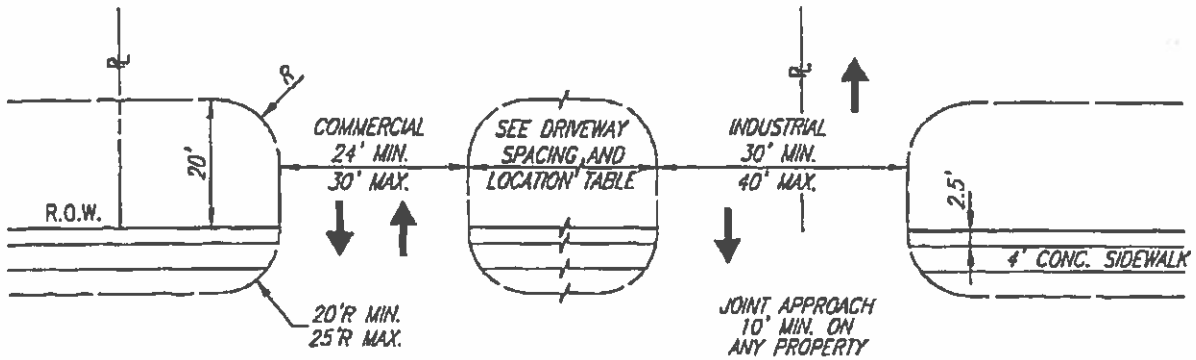
DRIVEWAYS WIDTH, RADIUS, SPACING
