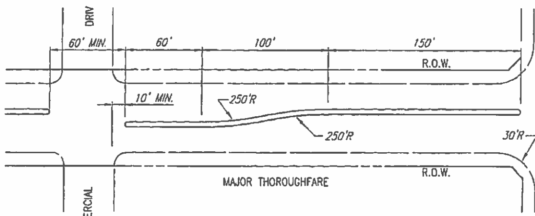
TYPICAL MEDIAN OPENING SPACING MAJOR THOROUGHFARE
