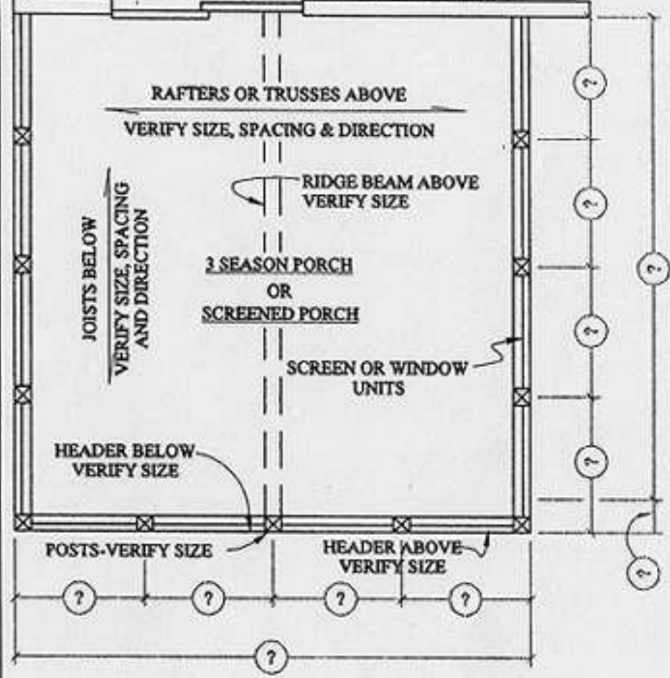
FLOOR PLAN 1/4" = 1'-0"
